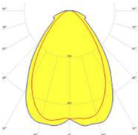
90° Light Beam
