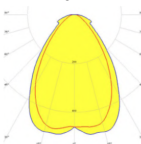
90° Light Beam
