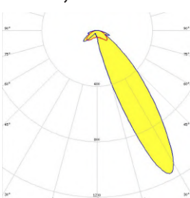
Asymmetric Beam
